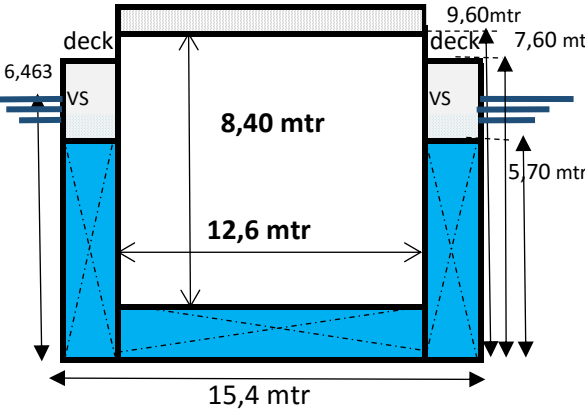
BULKHEAD POSITION 1
