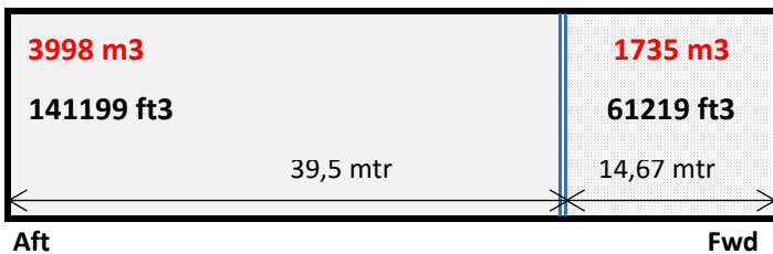
BULKHEAD POSITION 5
